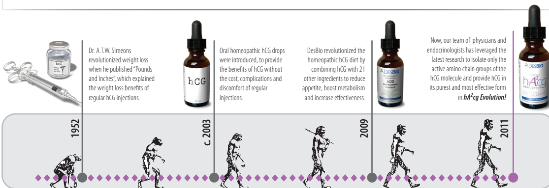
FIGURE 3: Active Chains in hA 2 cg
