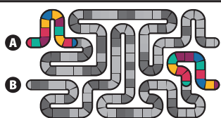
FIGURE 2: Active Portions of hCG
