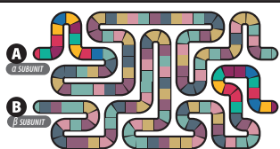
FIGURE 1: Entire hCG Molecule
